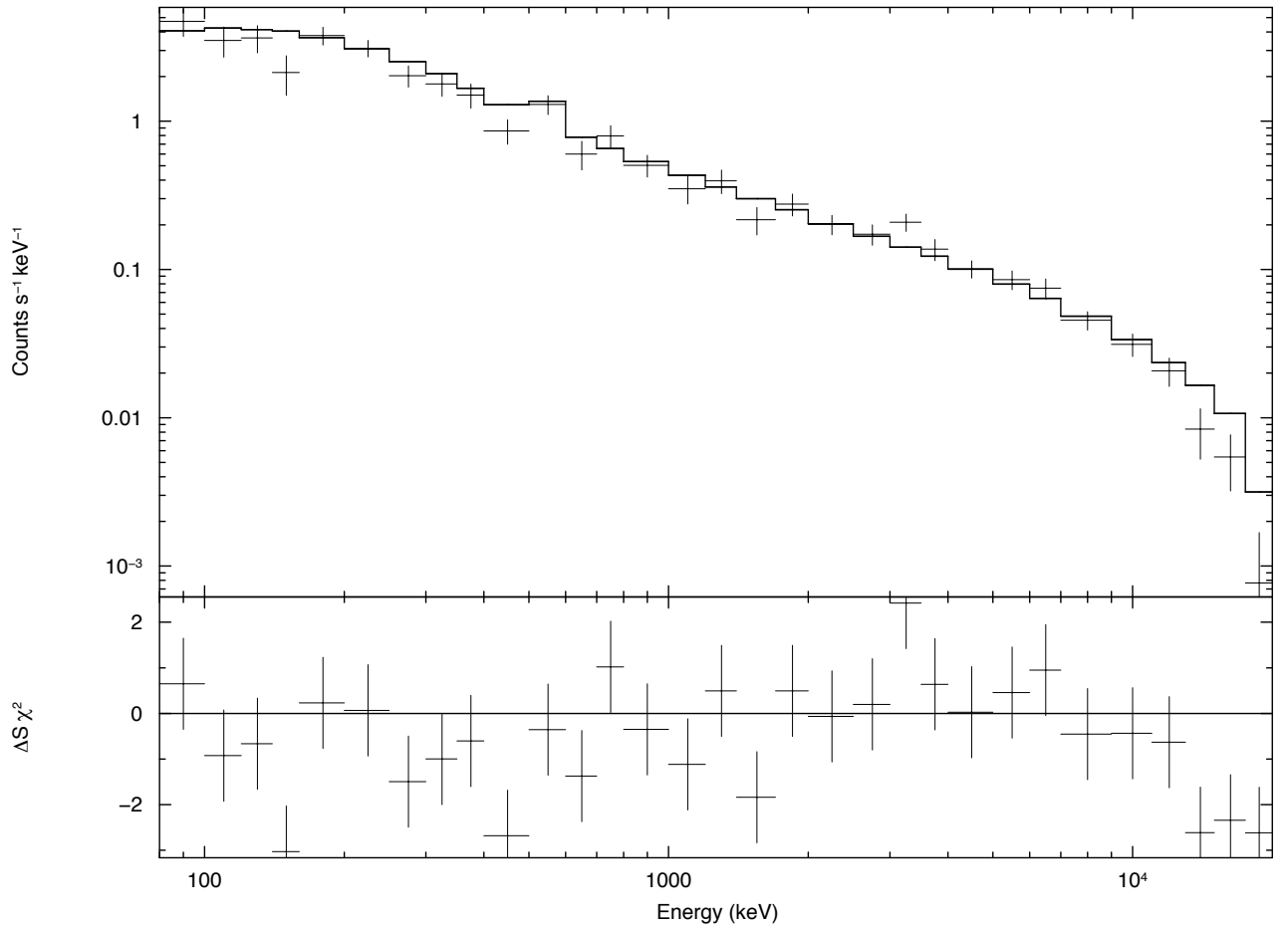
Figure 8. RHESSI experimental cumulative count spectrum for events triggered before 1 st January 2005 at latitudes lower than 2.5^\circ in absolute value. (top panel) Solid curve: the MCAL best fit model convolved with the RHESSI response matrix after the normalization factor is fit to RHESSI data (spectral parameters are kept constant). (bottom panel) The fit residuals.
