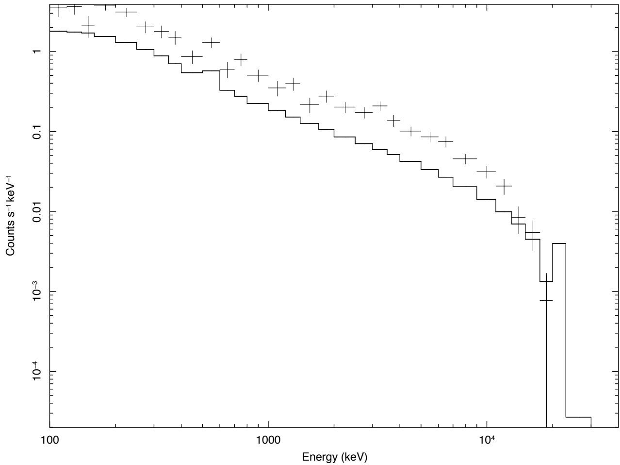
Figure 7. RHESSI experimental cumulative count spectrum for events triggered before 1 st January 2005 at latitudes lower than 2.5^\circ in absolute value. Solid curve: MCAL best fit model convolved with the RHESSI response matrix.
