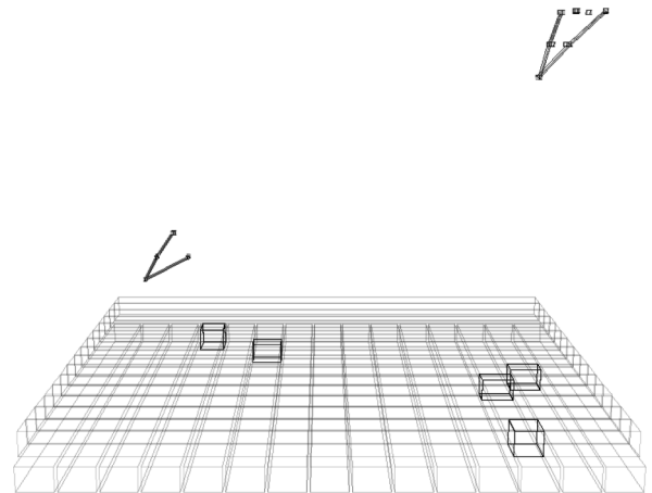
FIG. 2. 3D view of the tracks reconstructed for the two GRID events detected in association with TGF 12809-19. The MCAL detector with the detected events is shown at the bottom of the figure. The AGILE pointing direction is orthogonal to the MCAL detection planes, toward the top of the figure.
