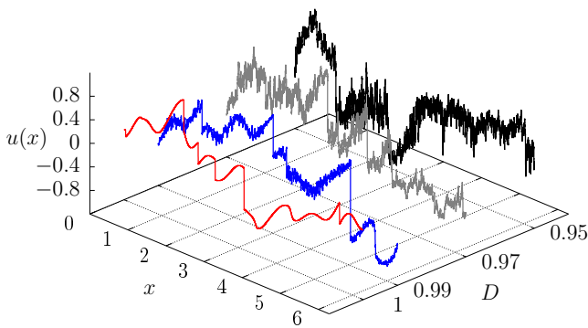
Fig. 1. Left: Snapshots of real space velocity profiles as a function of space and fractal Fourier dimension: D = 1 (red), D = 0.99 (blue), D = 0.97 (grey) and D = 0.95 (black). Right: Mean energy spectra in log-log scale, obtained for the same four fractal dimensions D and using the same colour code as in the left panel. The black solid line is the scaling slope k^{-2} produced by the undecimated ( D = 1.0 ) Burgers equation.
