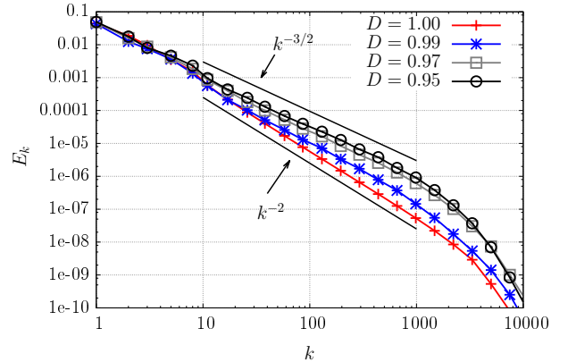
Fig. 1. Left: Snapshots of real space velocity profiles as a function of space and fractal Fourier dimension: D = 1 (red), D = 0.99 (blue), D = 0.97 (grey) and D = 0.95 (black). Right: Mean energy spectra in log-log scale, obtained for the same four fractal dimensions D and using the same colour code as in the left panel. The black solid line is the scaling slope k^{-2} produced by the undecimated ( D = 1.0 ) Burgers equation.
