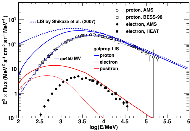
Figure 6. LIS of protons (thick blue line), and positrons (thin red line) used to calculate the \gamma -ray emissivity model in Figure 5 with a compilation of direct measurements at the Earth; see Alcaraz et al. (2000a), Sanuki et al. (2000), and Shikaze et al. (2007) for proton data and Alcaraz et al. (2000b) and Barwick et al. (1998) for electron data. Modulated spectrum with \phi = 450 MV is given by the thin blue line. The proton LIS adopted by Shikaze et al. (2007) is shown by the dotted blue line.
