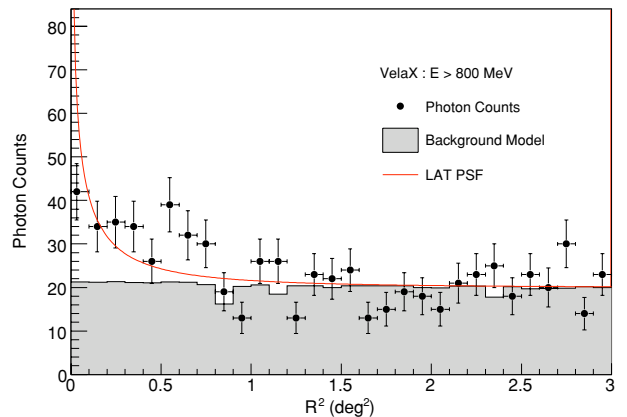
Figure 3. Radial profile of the LAT data about the best-fit position provided by Sourcelike for a point source (l, b) = (263^\circ:03, -3^\circ:27) as reported in Table 1 ( E > 800 MeV). The LAT PSF is overlaid as a red solid line for comparison. The background model is presented as a gray histogram and the black dots represent the LAT data.
