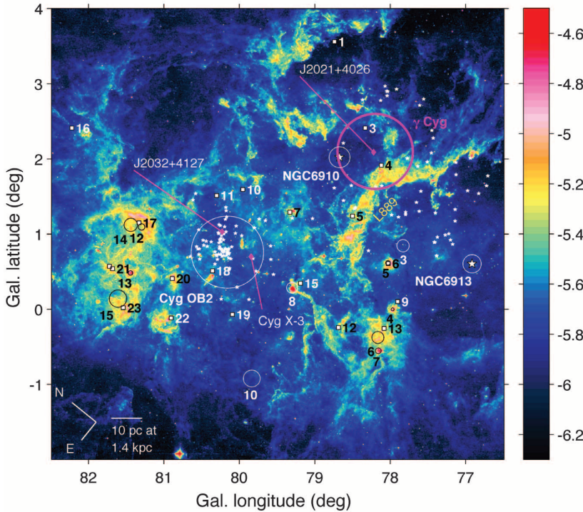
Fig. 1. An 8- \mu\text{m} intensity map of the Cygnus X region for MSX ( \text{W m}^{-2} \text{ sr}^{-1} , in log scale), outlining the PDRs. Objects are noted with their names or numbers: Cyg X-3 and pulsars J2021+4026 and J2032+4127 (magenta diamonds); the \gamma Cygni supernova remnant (magenta circle); OB associations [white or black circles (7)]; HII regions [white squares (10)]; and OB stars from Cyg OB2 and Cyg OB9 [white stars (8, 29)].
