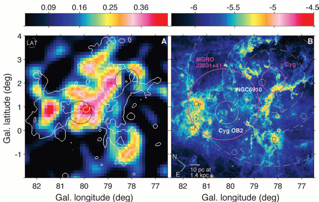
Fig. 3. (A) Photon count residual map in the 10- to 100-GeV band (30), smoothed with a \sigma = 0.25^\circ Gaussian kernel, and overlaid with the 10^{-5.6} \text{ W m}^{-2} \text{ sr}^{-1} white contour of the 8- \mu\text{m} intensity. The typical LAT angular resolution above 10 GeV is indicated. The black circles mark \gamma Cygni and Cyg OB2. (B) An 8- \mu\text{m} map and solid circles for \gamma Cygni and stellar clusters, as in Fig. 1. The large magenta circle marks the location and extent of the source MGRO J2031+41 (14); dashed circles give upper limits to the diffusion lengths of 10, 10^2 , and 10^3 GeV particles after 5000 years of travel time using the standard interstellar diffusion coefficient. Their origin from the position of the rim of \gamma Cygni 5000 years ago is purely illustrative.
