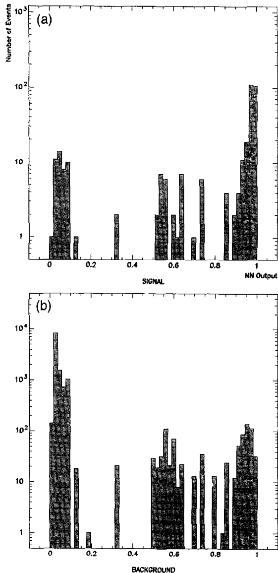
Fig. 3. The neural network output for TRD (a) signal and (b) background events selected with high purity by means of the time-of-flight, spectrometer and calorimeter.
