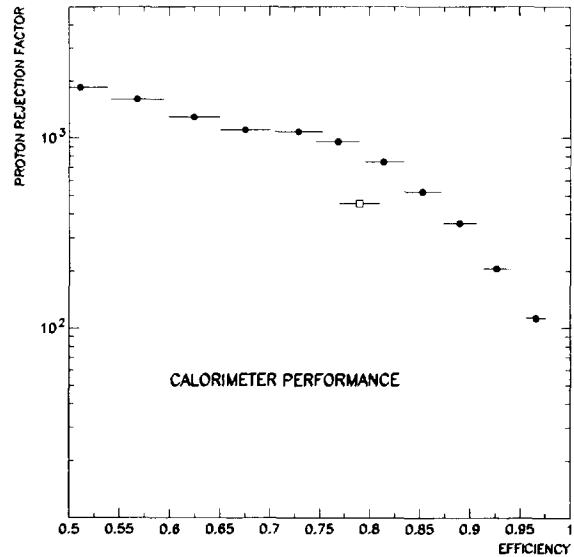
Fig. 6. Proton rejection factor versus signal efficiency of the Calorimeter on flight data (black circles); the result of the conventional analysis (Ref. [13,14]) is also drawn (white box).
