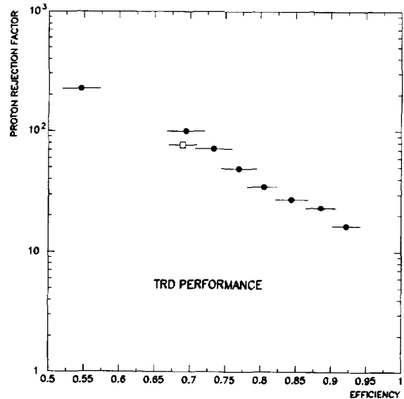
Fig. 4. Proton rejection factor versus signal efficiency of the TRD on flight data (black circles); the result of the conventional analysis (Ref. [13,15]) is also drawn (white box).
