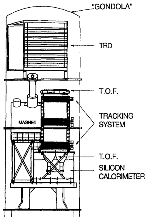
Fig. 1. The New Mexico State University balloon-borne magnet facility equipped with Wizard-TS93 apparatus used for the 1993 flight to identify cosmic ray electrons and positrons in the energy range from 5 to 50 GeV.
