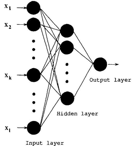
Fig. 2. The three-layered feed-forward neural network classifier used to select electrons and positrons detected with the TRD and Calorimeter.
