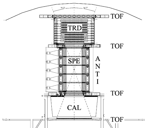
Fig. 1. The PAMELA telescope (1050 mm high) consists of a transition radiation detector (TRD), a magnetic spectrometer equipped with silicon micro-strip detector (SPE), a silicon/tungsten calorimeter (CAL), a time-of-flight detector (TOF), and an anti-coincidence system (ANTI).
