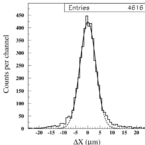
Fig. 3. Spatial resolution of the X view.
