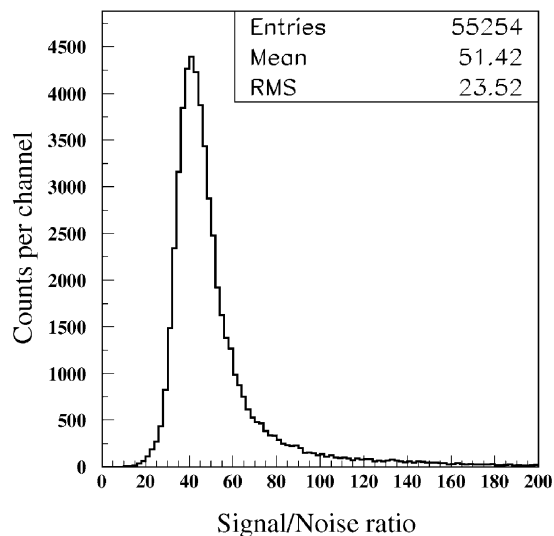
Fig. 2. S/N ratio of the X tracker view.
