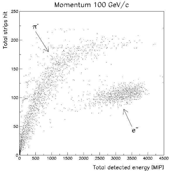
Fig. 4. Separation between electrons and pions (both with momentum 100 GeV/c) in the calorimeter, obtained reporting the number of hit strips as a function of the total energy deposition.
