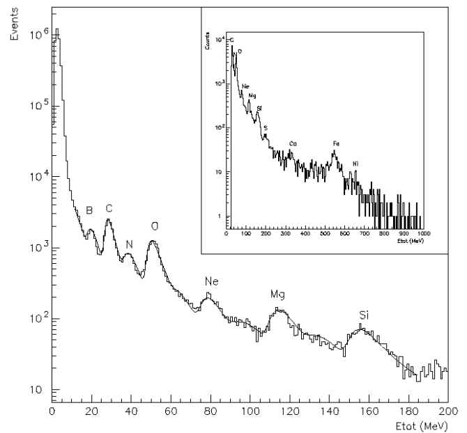
Fig. 2. Nuclear identification capabilities of SilEye-2 for nuclei up to Si. In the inset is shown the contribution of nuclei up to Ni. The continuous line corresponds to a fit using a Landau distribution per nuclear species (see text).
