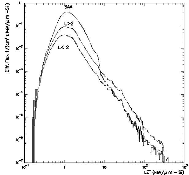
Fig. 4. Linear Energy Transfer in silicon for solar quiet period measured with SilEye-2 (solar quiet sessions between August 1998 and August 1999). Top: SAA region. Center: galactic ( L > 2 ) region. Bottom: remaining region ( L < 2 , outside the SAA).
