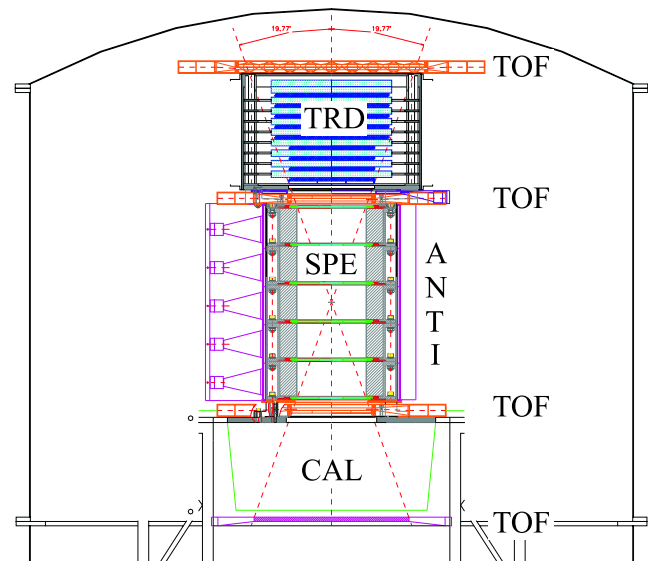
Figure 1: A section of the PAMELA instrument
