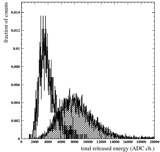
Fig. 5. Distributions of total energy released in the TRD for electrons (shaded region) and pions, both with momentum of 40 GeV/c.
