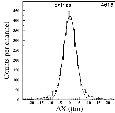
Fig. 3. Spatial resolution of the X view.
