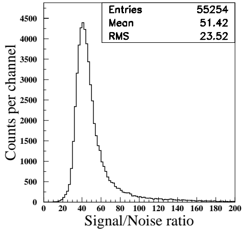
Fig. 2. S/N ratio of the X tracker view.
