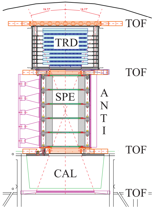
Fig. 1. The PAMELA telescope (1050 mm high) consists of a transition radiation detector (TRD), a magnetic spectrometer equipped with silicon micro-strip detector (SPE), a silicon/tungsten calorimeter (CAL), a time-of-flight detector (TOF), and an anti-coincidence system (ANTI).
