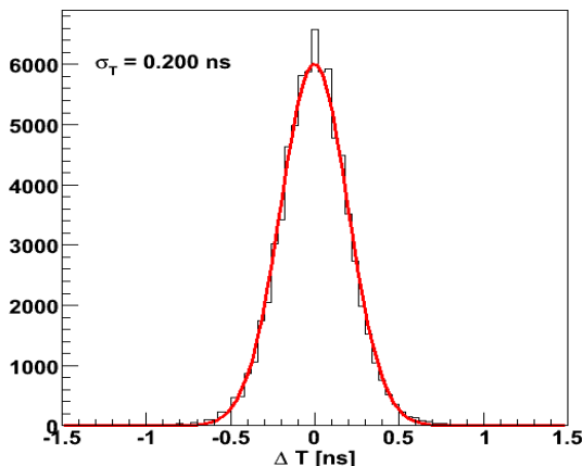
Figure 3: Timing resolution of a single S11 paddle for protons
