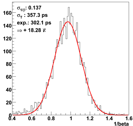
Figure 5: ToF resolution of one S11-S31 combination for protons
