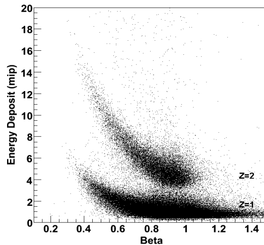
Figure 7: Charge bands for flight data measured by one photomultiplier in a S2 scintillator
