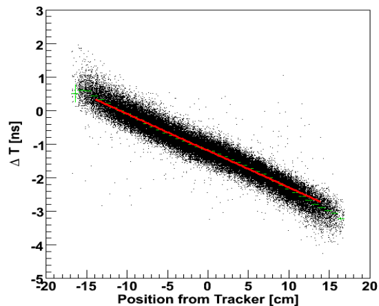
Figure 2: Position of the incident particle from timing vs. position from particle trajectory
