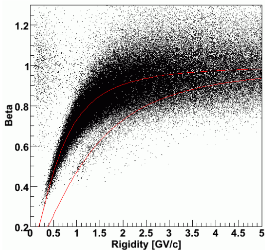
Figure 6: Beta versus rigidity plot for Z=1 particles. The solid lines show the expected behaviour for protons and deuterium
