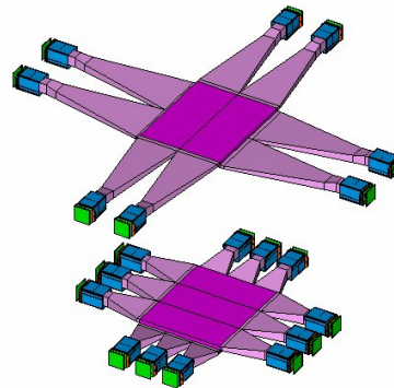
Figure 1: The PAMELA time-of-flight system
