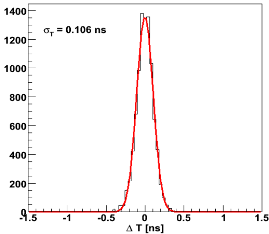
Figure 4: Timing resolution of a single S11 paddle for helium
