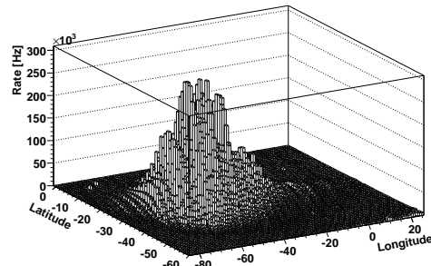
Figure 4: Singles rates (Hz) in the CAS1 detector as function of the orbital position averaged on several orbits traversing the SAA from South to North. The figure shows a detail of the rates in the vicinity of the SAA. Each bin in the histogram corresponds to the average rate in a 1 square degree.
