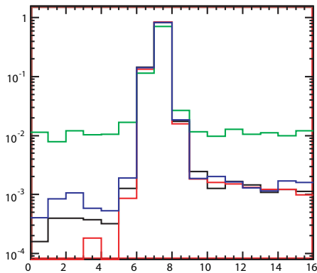
Figure 1: Shift register contents as function of the orbital position. Data are shown only for the channels connected to the main board for polar regions (black lines), equatorial regions (red), SAA (green) and electron belts (blue). All histograms are normalised to unit area.
