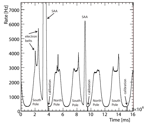
Figure 2: Singles rates (Hz) in the CAS1 detector as function of time. The peak out of scale reaches a rate of 71.4 kHz and is due to a passage of PAMELA through the SAA. The smaller peaks correspond to the passage in the electron belts.
