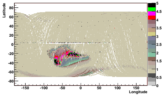
Figure 5: Ratio of the singles rates CAS4/CAS3 as function of the geographical latitude and longitude for all the runs where the satellite crosses the SAA moving northwards.
