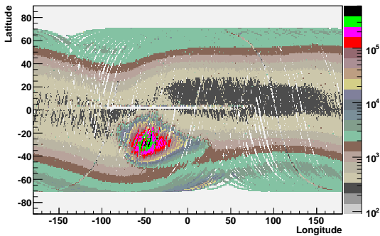
Figure 3: Singles rate (Hz) in the CAS1 detector as function of the geographical latitude and longitude for several runs. See text for details.
