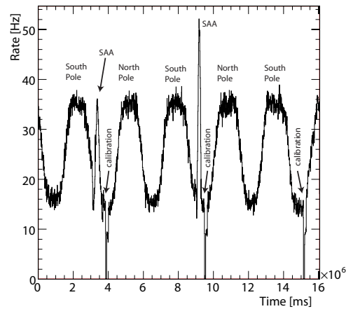
Figure 6: PAMELA trigger rate along 3 consecutive orbits.
