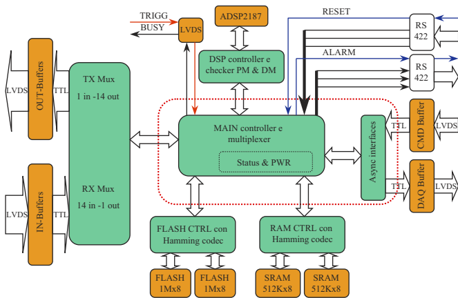
Fig. 1. IDAQ functional block scheme.
