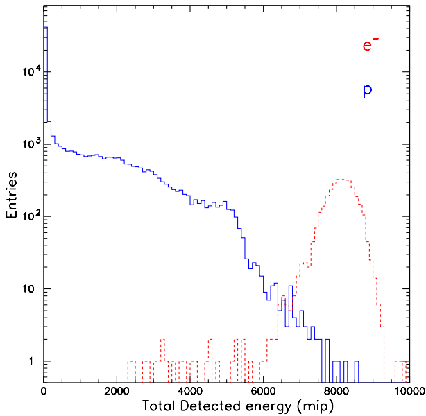
Fig. 4. An illustration of electron–proton separation using a simple total deposited energy variable. The test beam data were collected for particles of momentum 50 GeV/c. After a cut placed at 7300 mip 14 protons (99.98% reduction) and 3197 electrons (4.3% reduction) remain.
