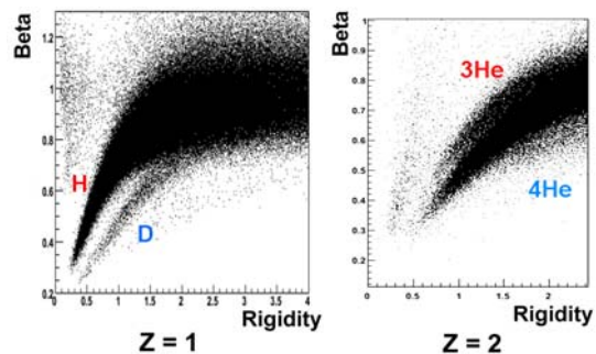
Fig 6: Mass separation for Z=1 and Z=2 particles with the \beta vs. rigidity method.
