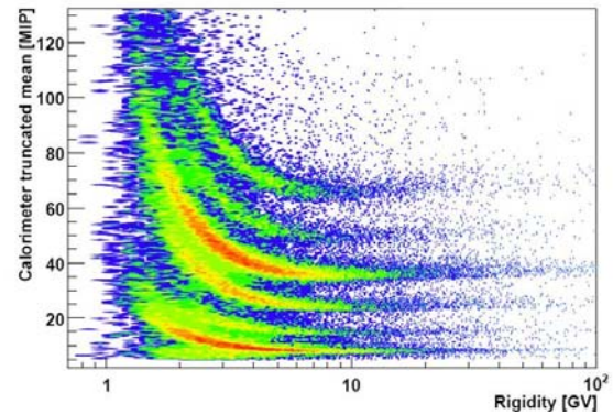
Fig 5: The ionization loss in the calorimeter with truncated mean using three points and at least four dE/dx measurements versus rigidity.
