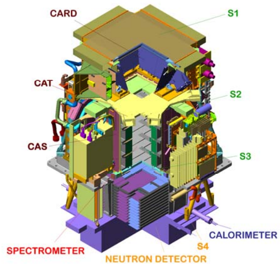
Fig 1. Schematic overview of the PAMELA apparatus. The detector is approximately 1.3 m high, has a mass of 470 kg and an average power consumption of 355 W.
