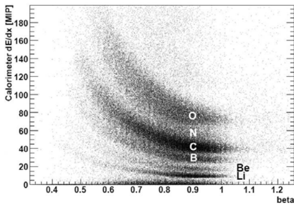
Fig 4: The ionization loss in the first plane of the calorimeter vs. the particle velocity.
