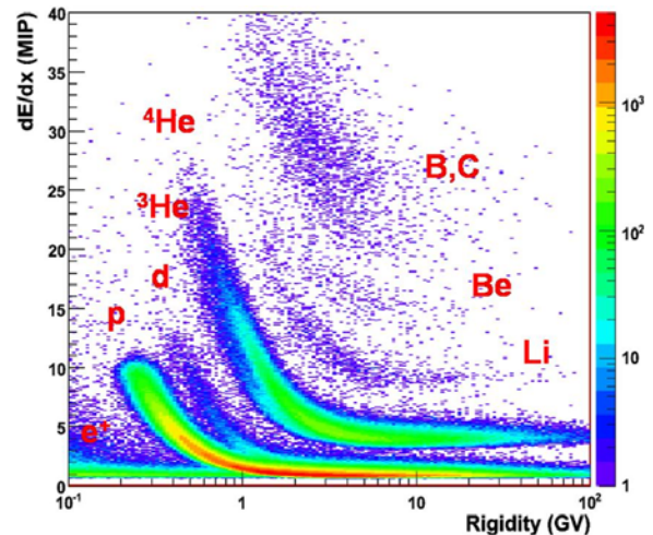
Fig. 3: The ionization loss in the tracker vs. rigidity.
