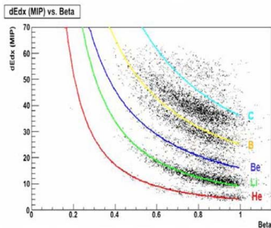
Fig. 2: Charge separation obtained with one of the S12 scintillators, illustrated by plotting the ionization energy loss vs. the particle velocity. The solid curves show the theoretical behavior.
