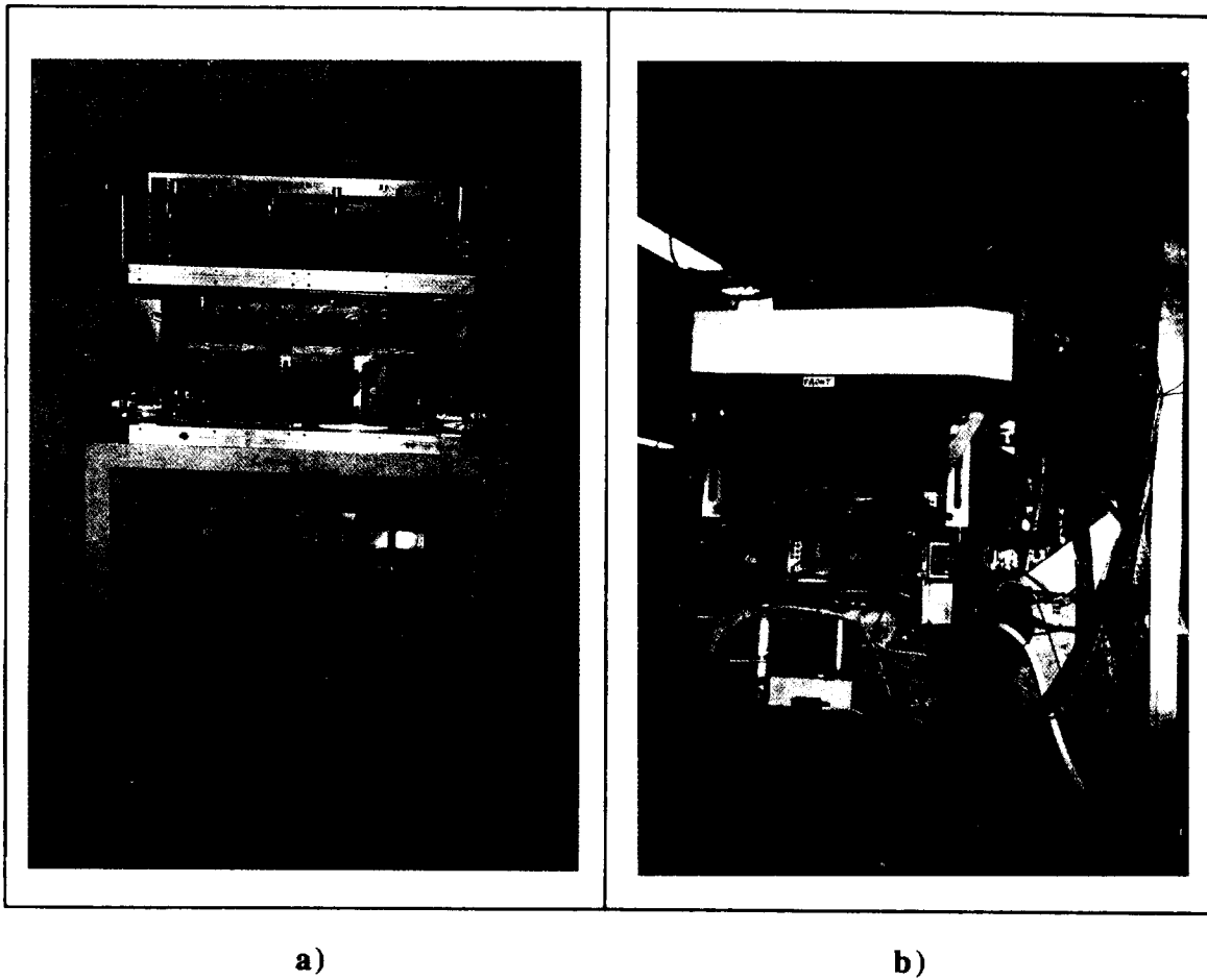
Figure 4 – Photographies of the complete arrangement of the calorimeter with its cooling box and the dedicated CAMAC Crate. a): stand-alone configuration without the cover; b) flight configuration in the payload; above the calorimeter stands the superconducting magnet.
