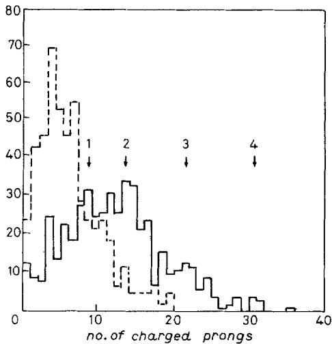
Fig. 3. - Distribution of the number of charged prongs produced by antihelium (solid line) in the WiZard calorimeter ( i.e. in the first module of the «full containment» calorimeter) compared with that for helium (broken line) at the same total energy (20 GeV). The arrows indicate the multiplicity regions of the number of annihilation vertices.
