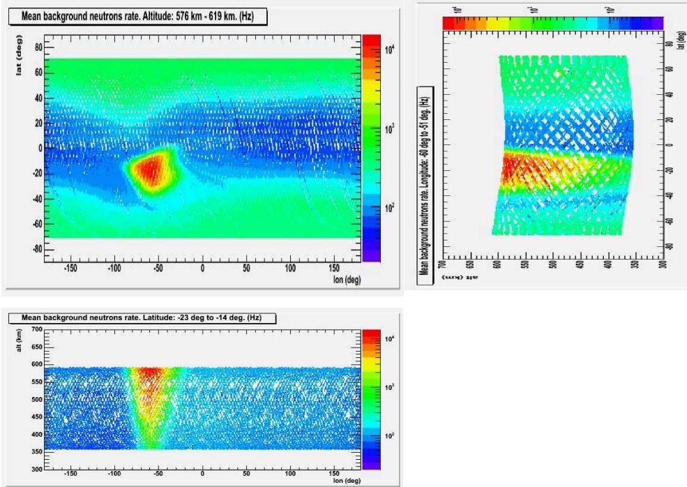
Figure 1: Counting rate of neutrons as function of latitude- longitude (altitude of 576-619 km, top left panel); altitude-latitude (longitude of 60^{\circ}W-51^{\circ}W , top right panel) and latitude-longitude (latitude of 23^{\circ}S-14^{\circ}S , lower left panel).
